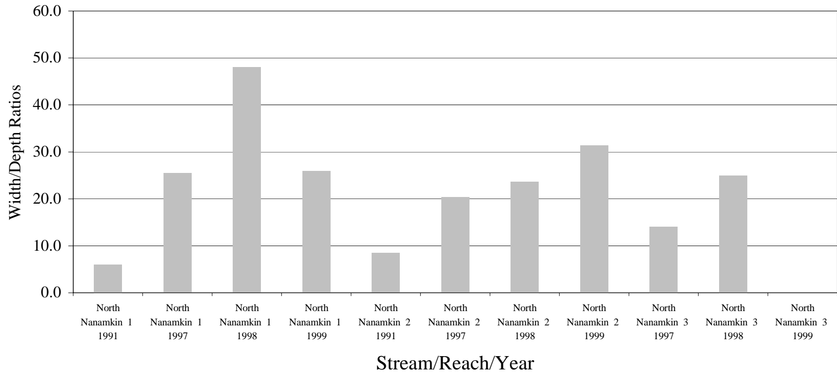
Chart 45. Width/Depth Ratios 1990-1999, North Nanamkin Creek
