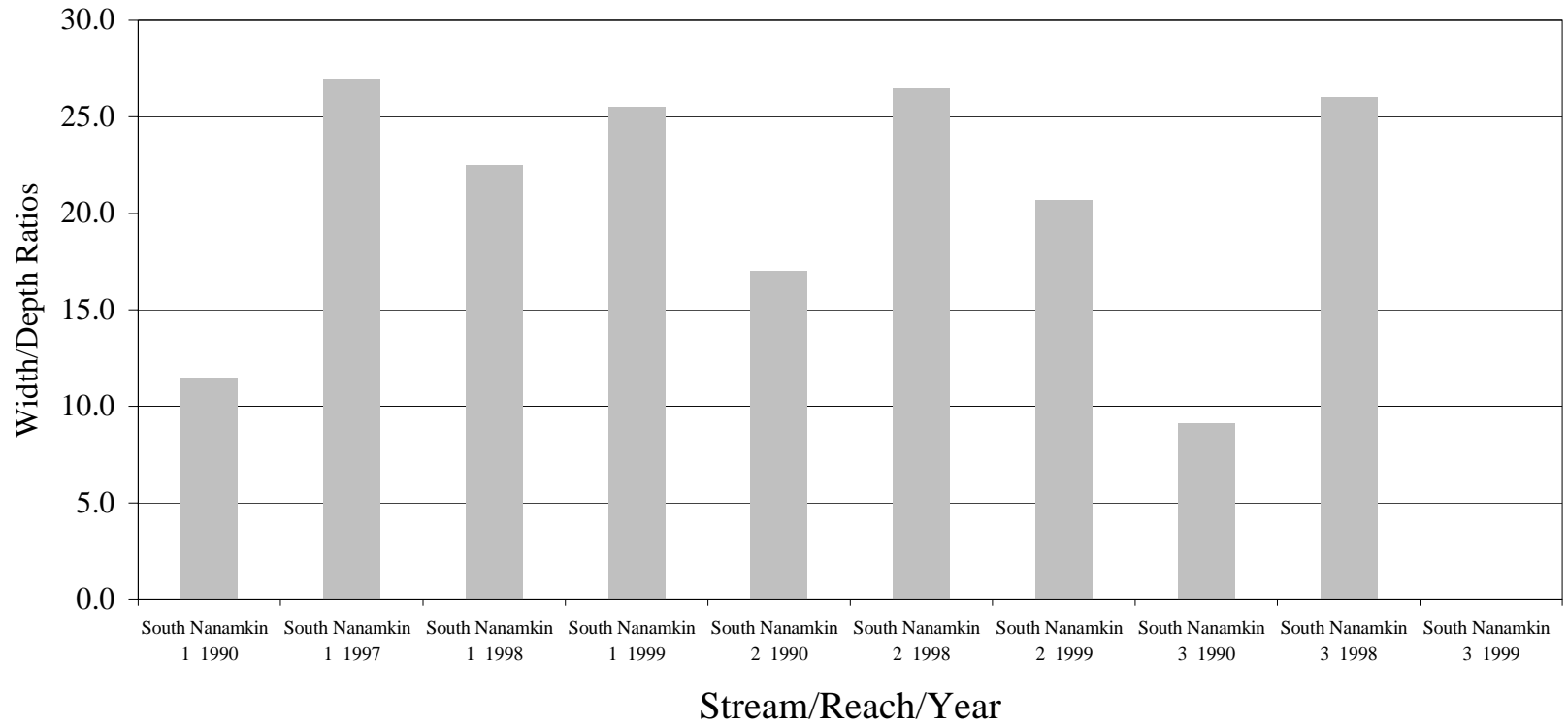
Chart 46. Width/Depth Ratios 1990-1999, South Nanamkin Creek
