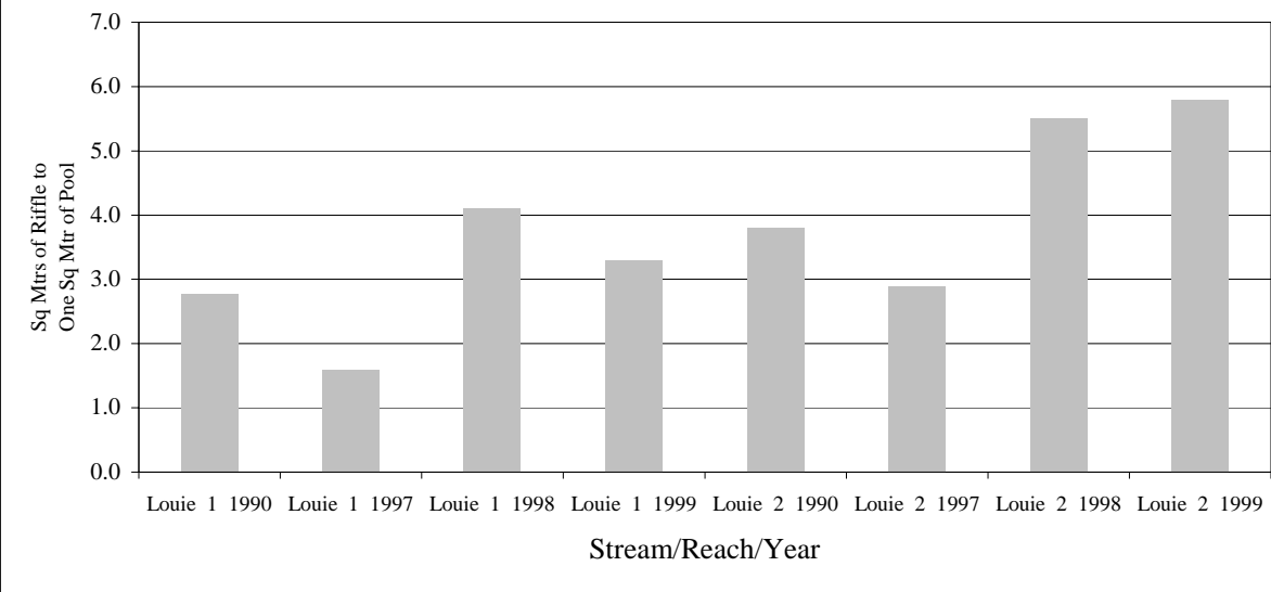
Chart 29. Pool-Riffle Ratios 1990-1999, Louie Creek
