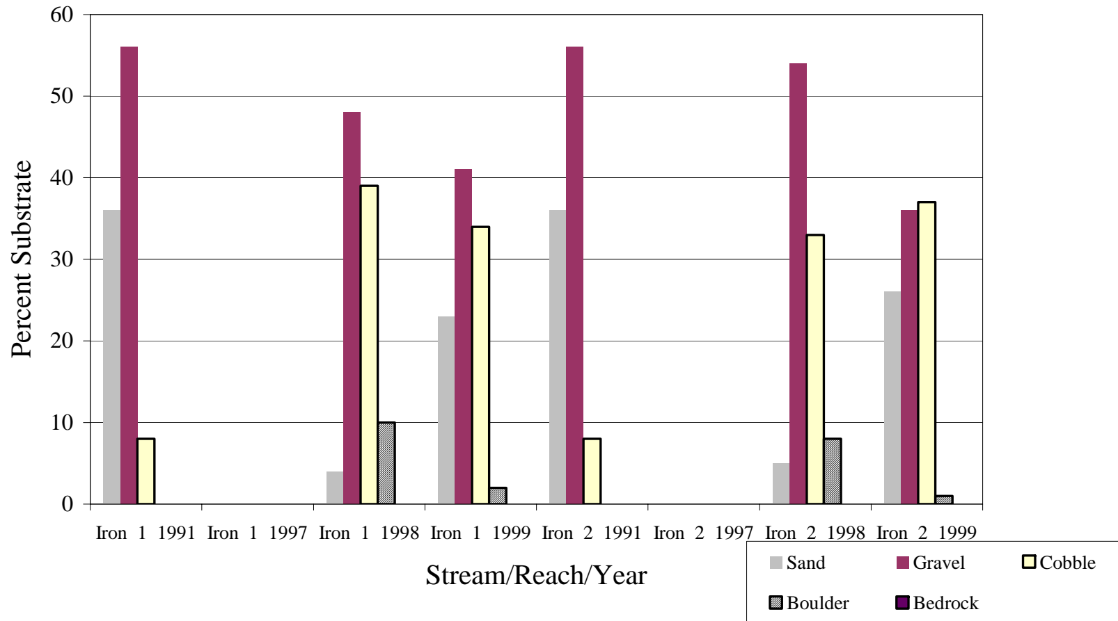
Chart 38. Percent Substrate 1990-1999, Iron Creek
